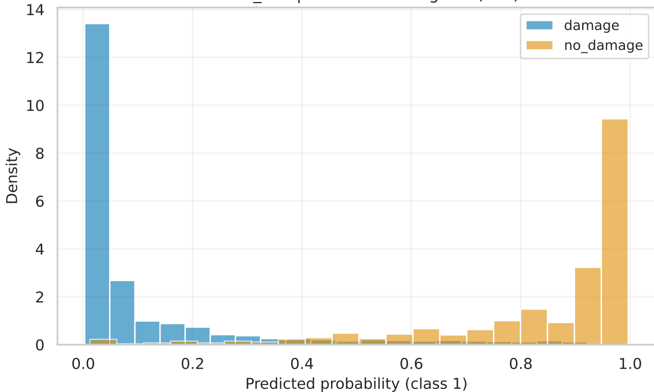
custom_cnn | val Score Histogram (raw)
