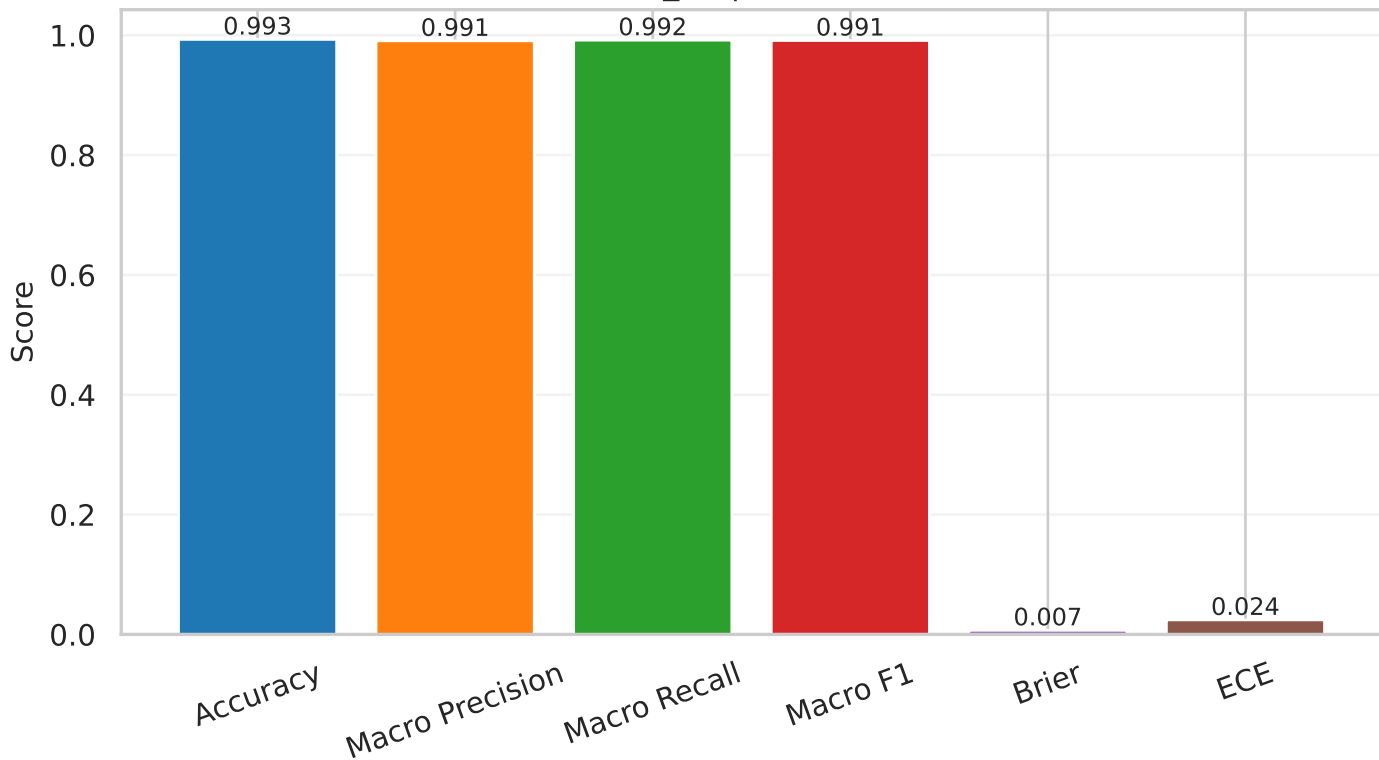
efficientnet_b1 | val (raw) metrics
