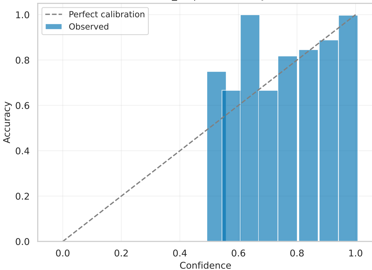
efficientnet_b1 | val Reliability (raw)
