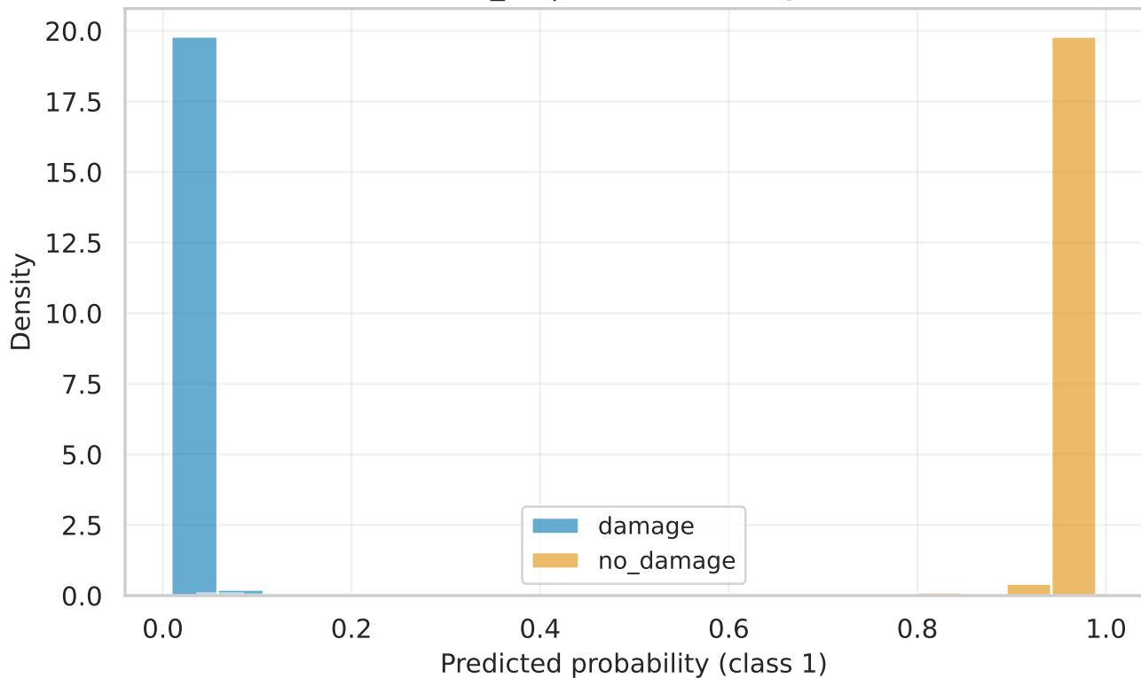
efficientnet_b1 | val Score Histogram (raw)
