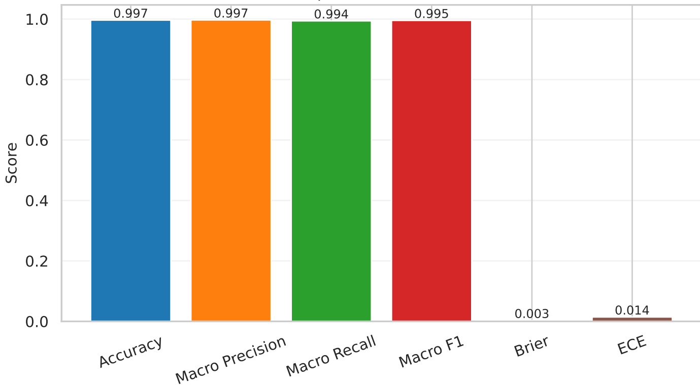
resnet18 | test (calibrated) metrics
