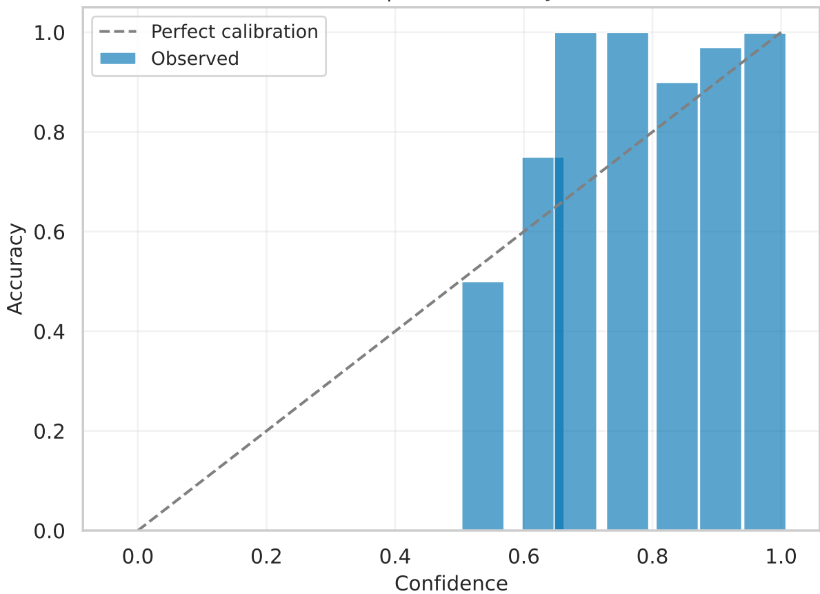
resnet18 | test Reliability (raw)
