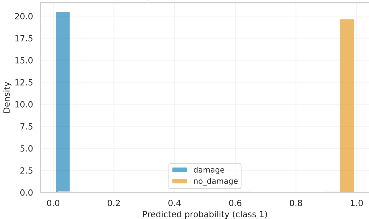
resnet50 | test Score Histogram (calibrated)
