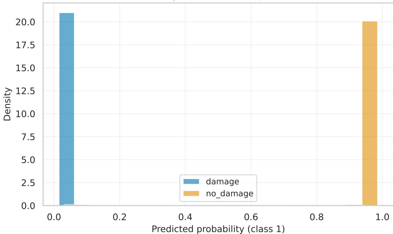
resnet50 | test Score Histogram (raw)
