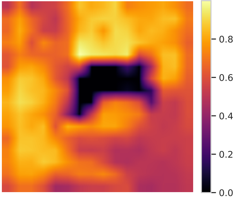
CAM
