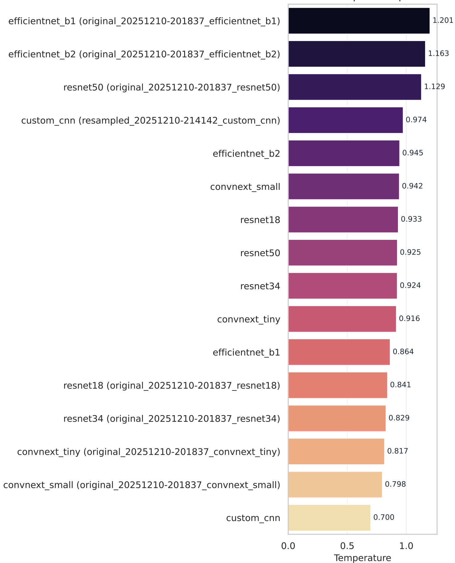
Calibration temperature per model
