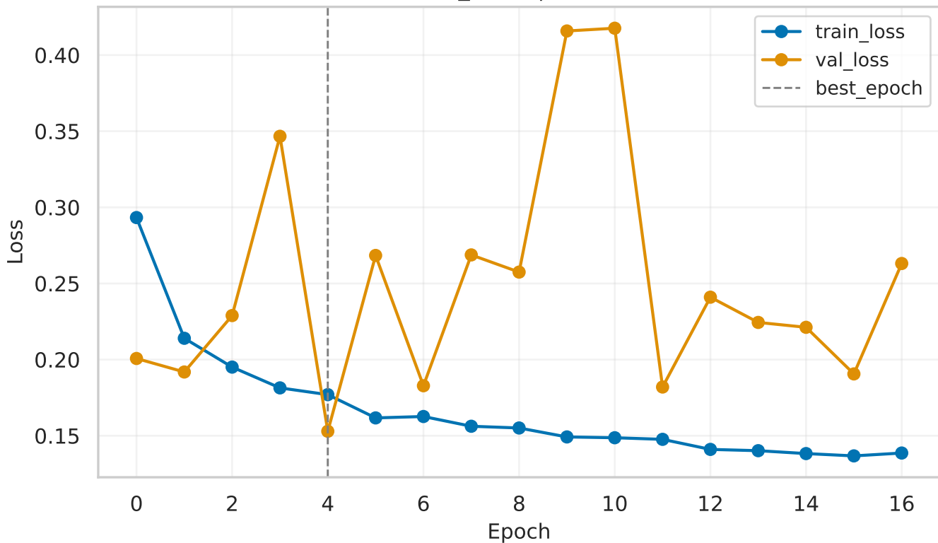
convnext_small | Loss curves
