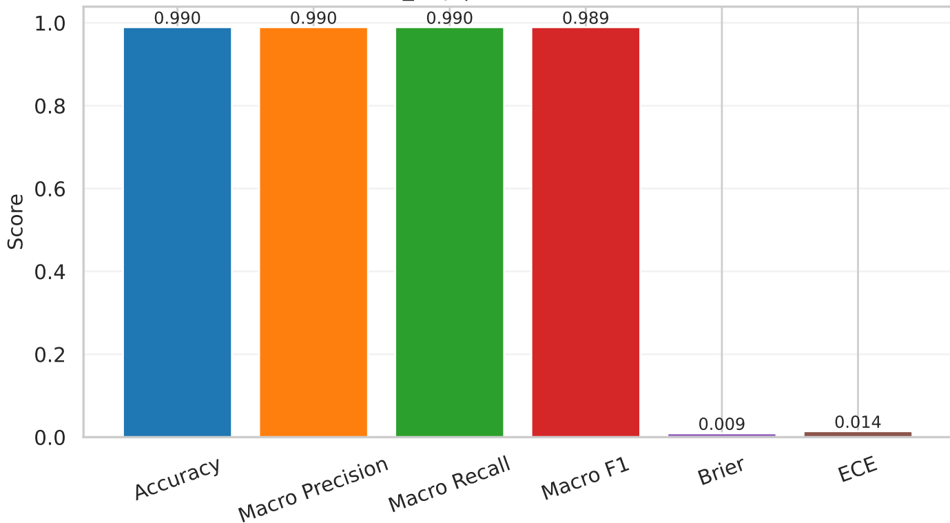
convnext_tiny | val (calibrated) metrics
