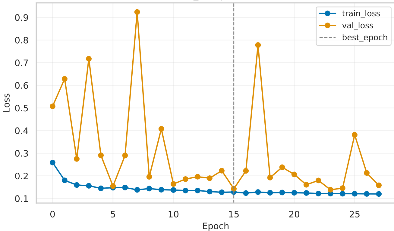
convnext_tiny | Loss curves
