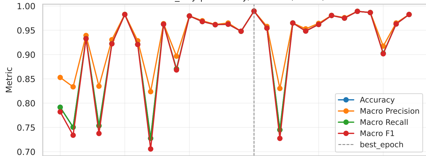
convnext_tiny | Accuracy/Precision/Recall/F1
