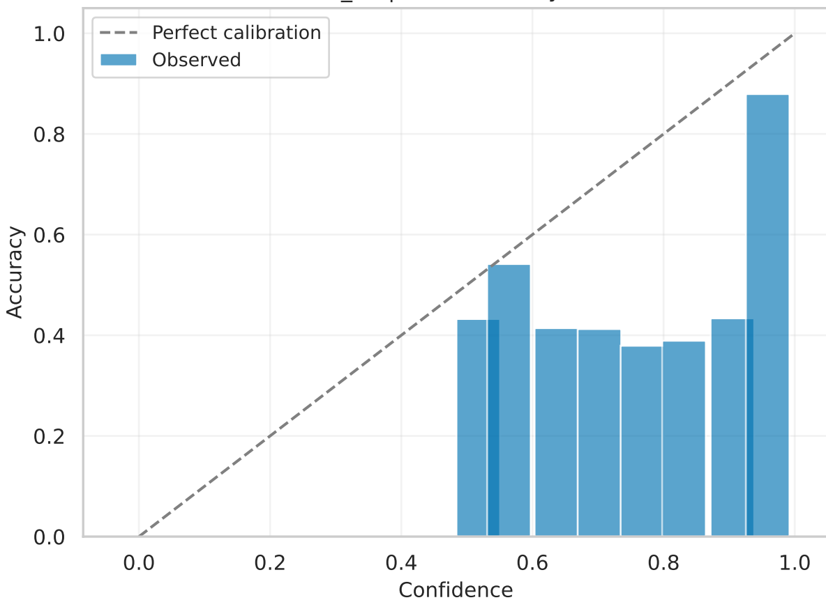
efficientnet_b1 | test Reliability (calibrated)
