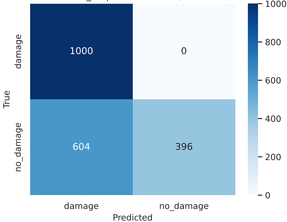
efficientnet_b1 | val Confusion (calibrated)
