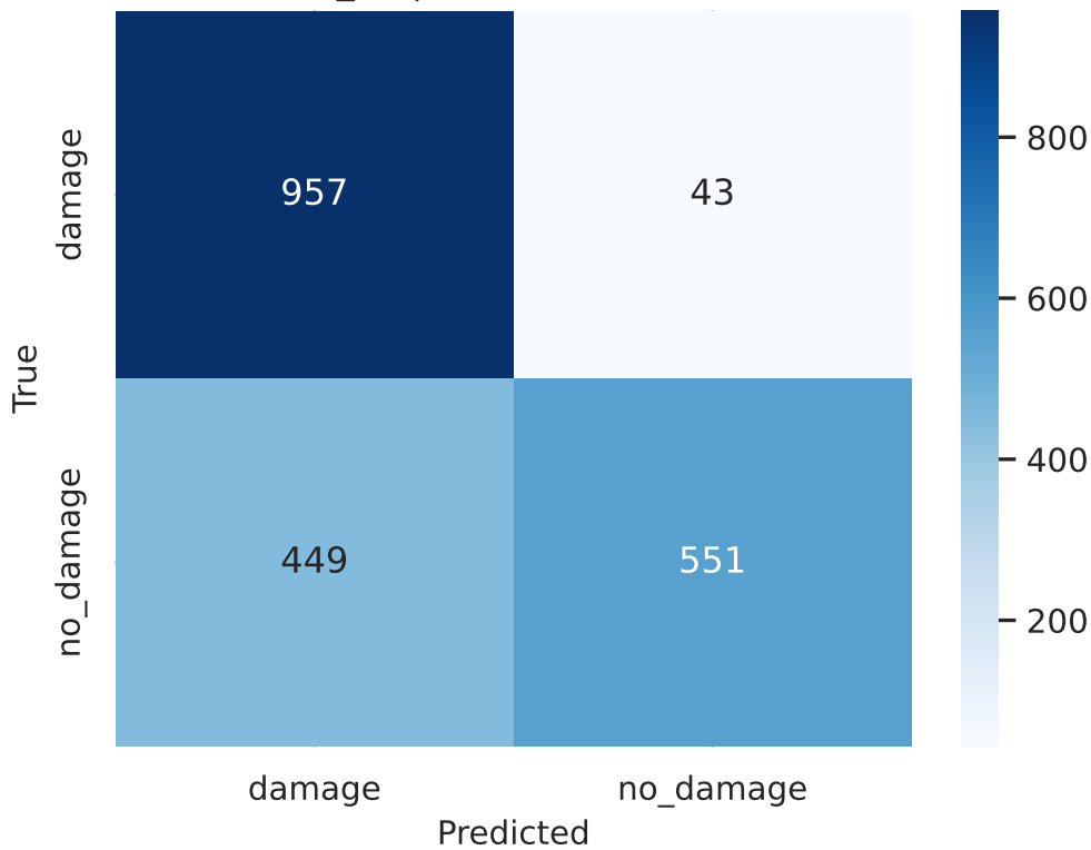
efficientnet_b2 | val Confusion (calibrated)
