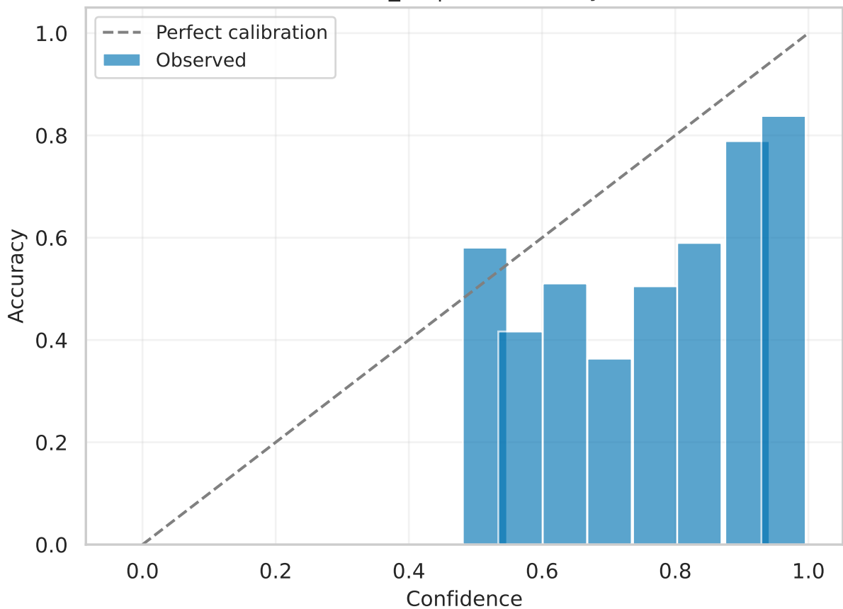
efficientnet_b2 | val Reliability (raw)
