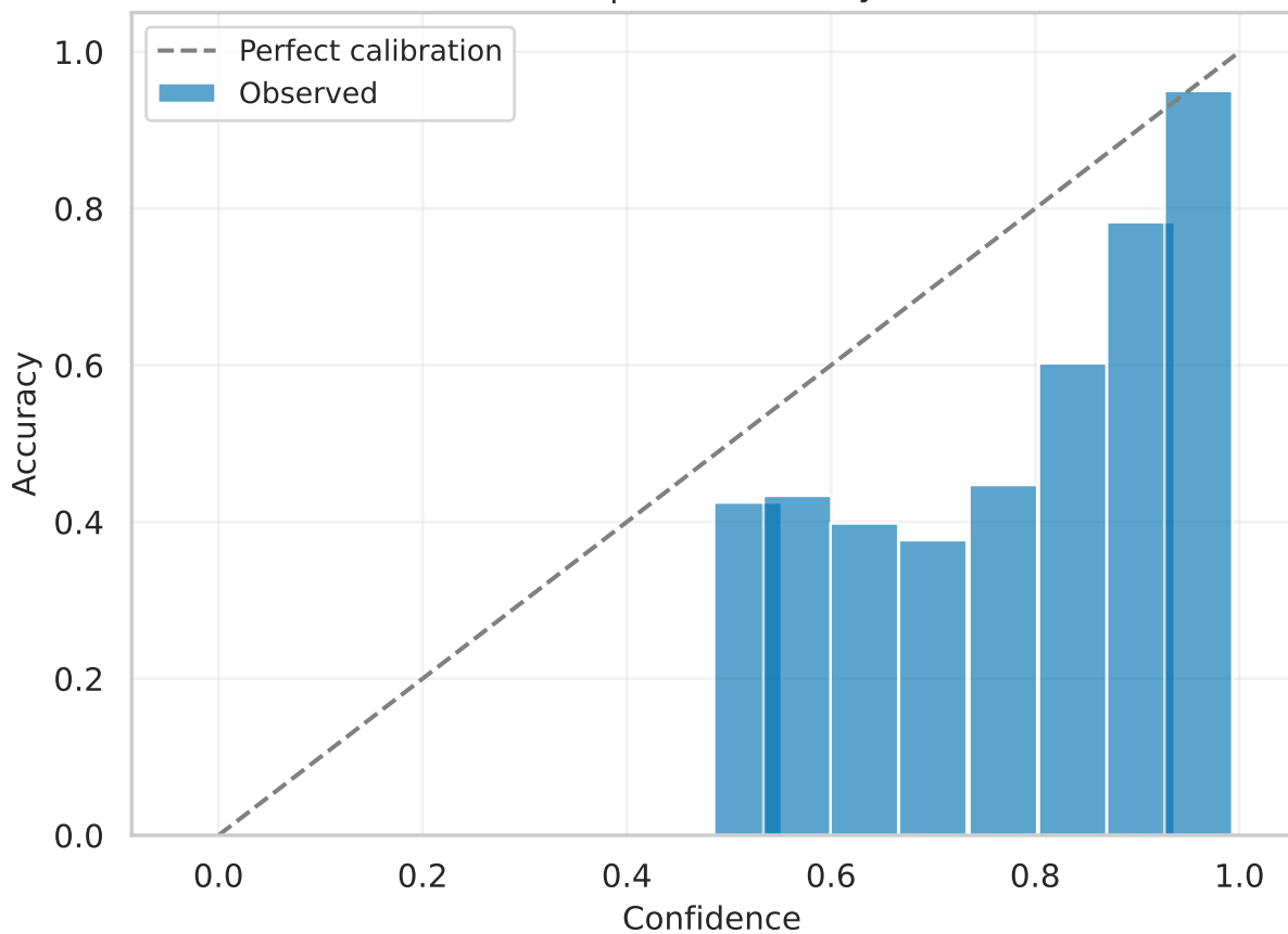
resnet50 | test Reliability (raw)
