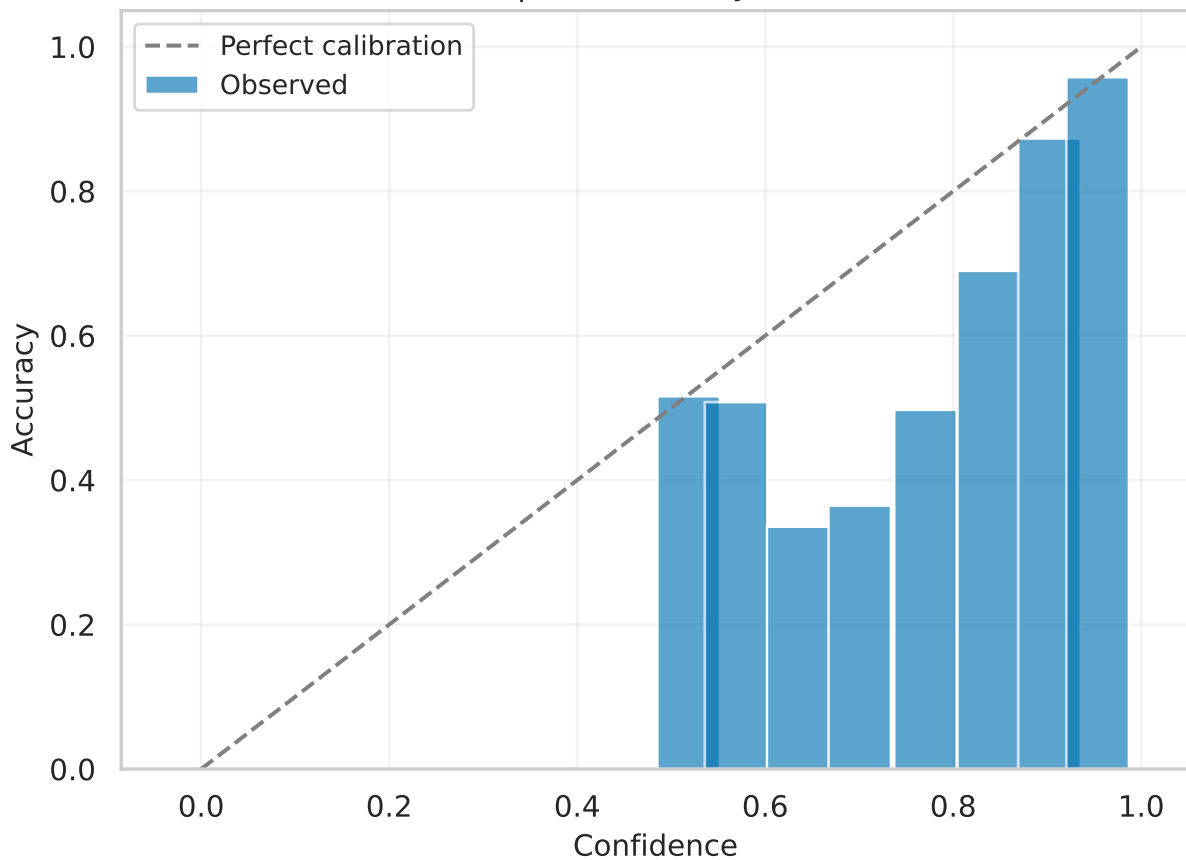
resnet50 | val Reliability (calibrated)
