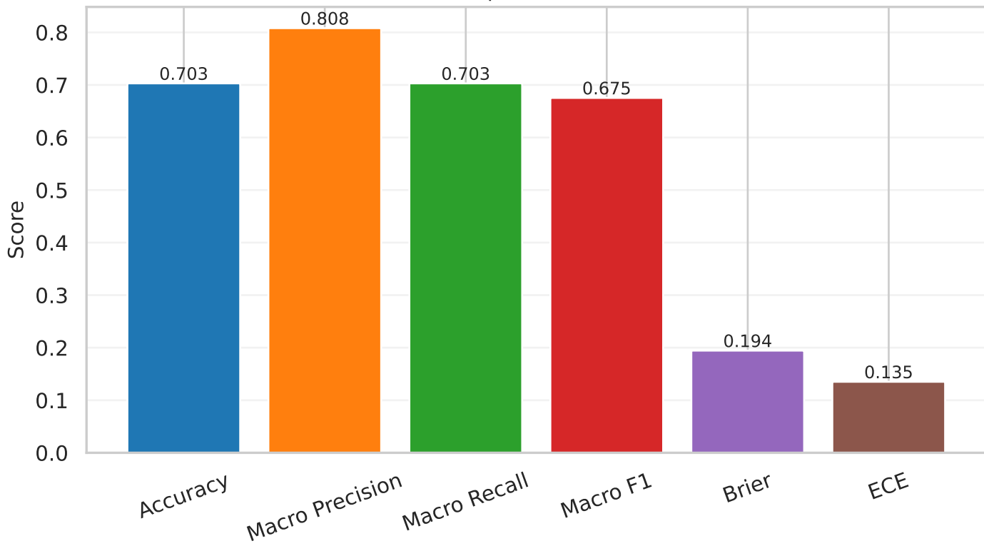
resnet50 | val (raw) metrics
