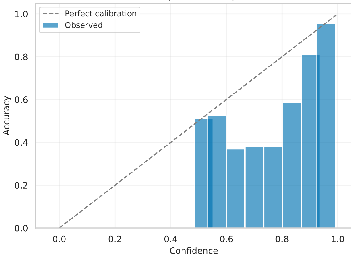
resnet50 | val Reliability (raw)
