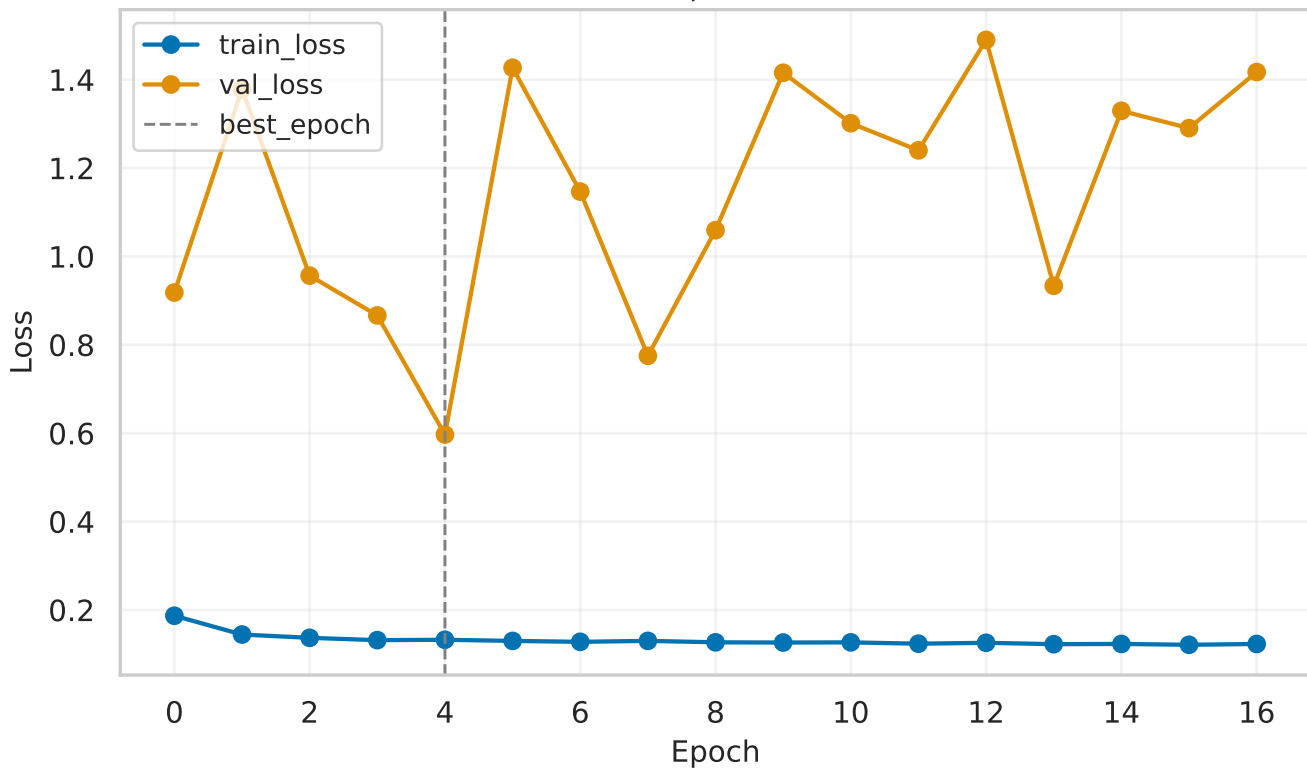
resnet50 | Loss curves
