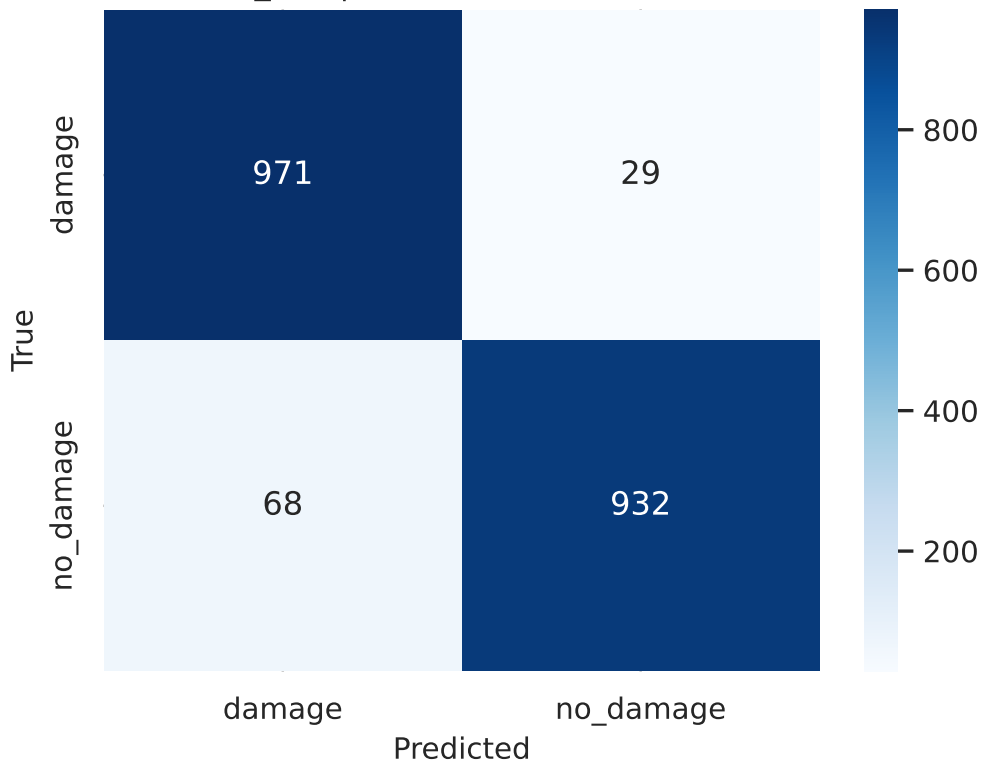
custom_cnn | test Confusion (calibrated)
