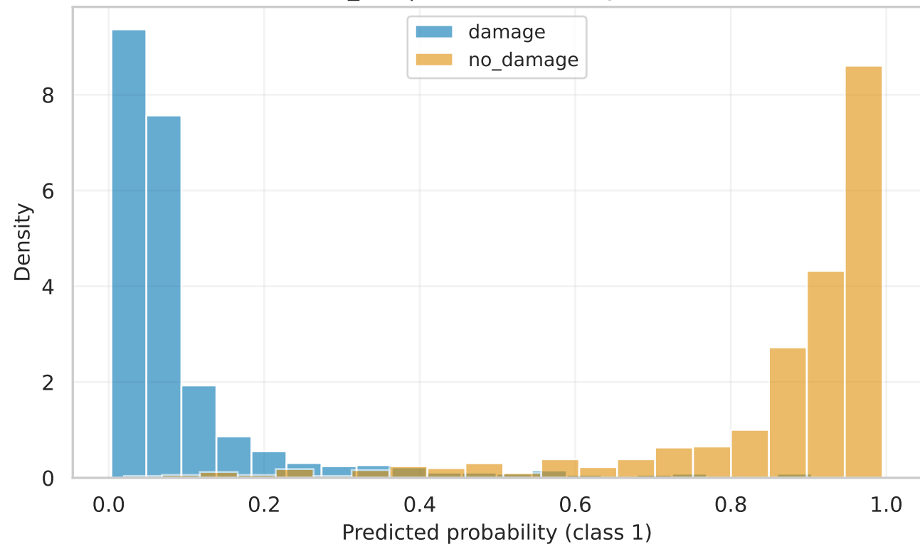
custom_cnn | test Score Histogram (raw)
