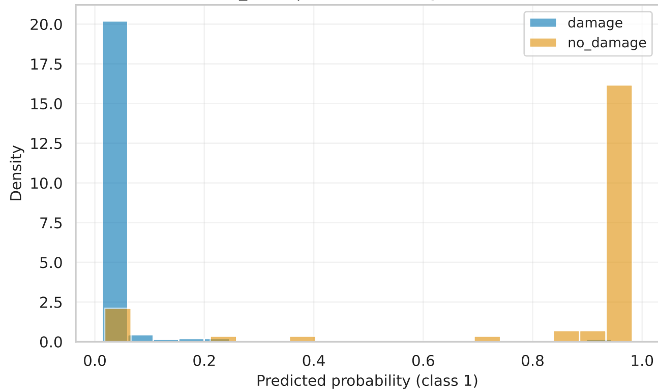
convnext_small | val Score Histogram (calibrated)
