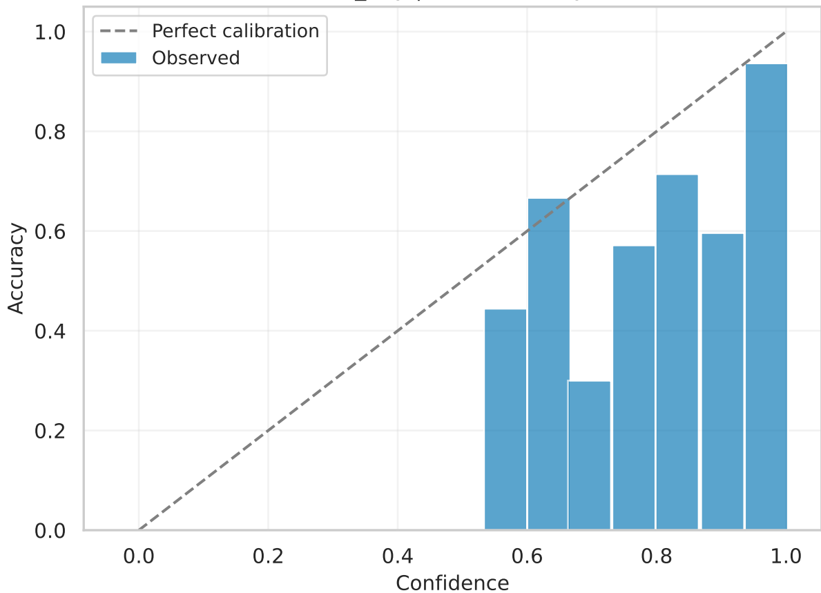
convnext_tiny | test Reliability (raw)
