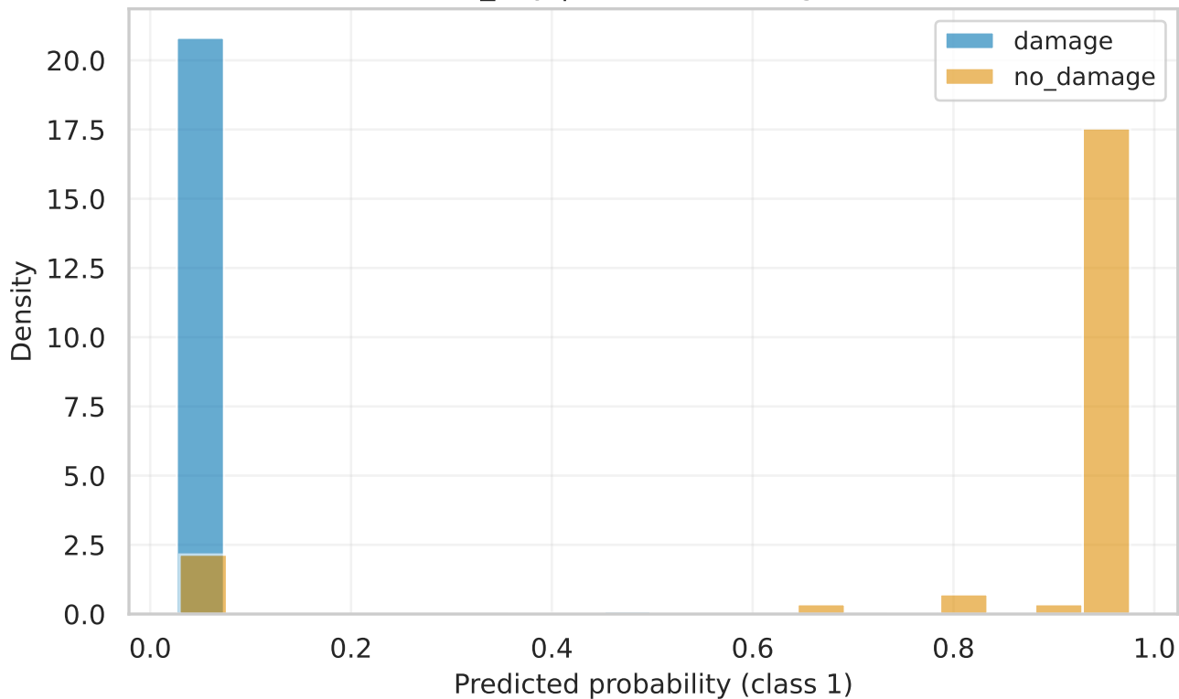
convnext_tiny | val Score Histogram (raw)
