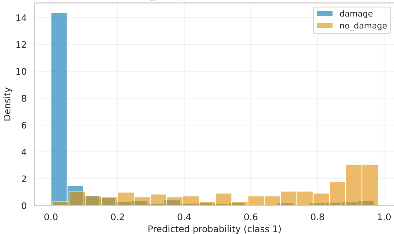
custom_cnn | test Score Histogram (raw)
