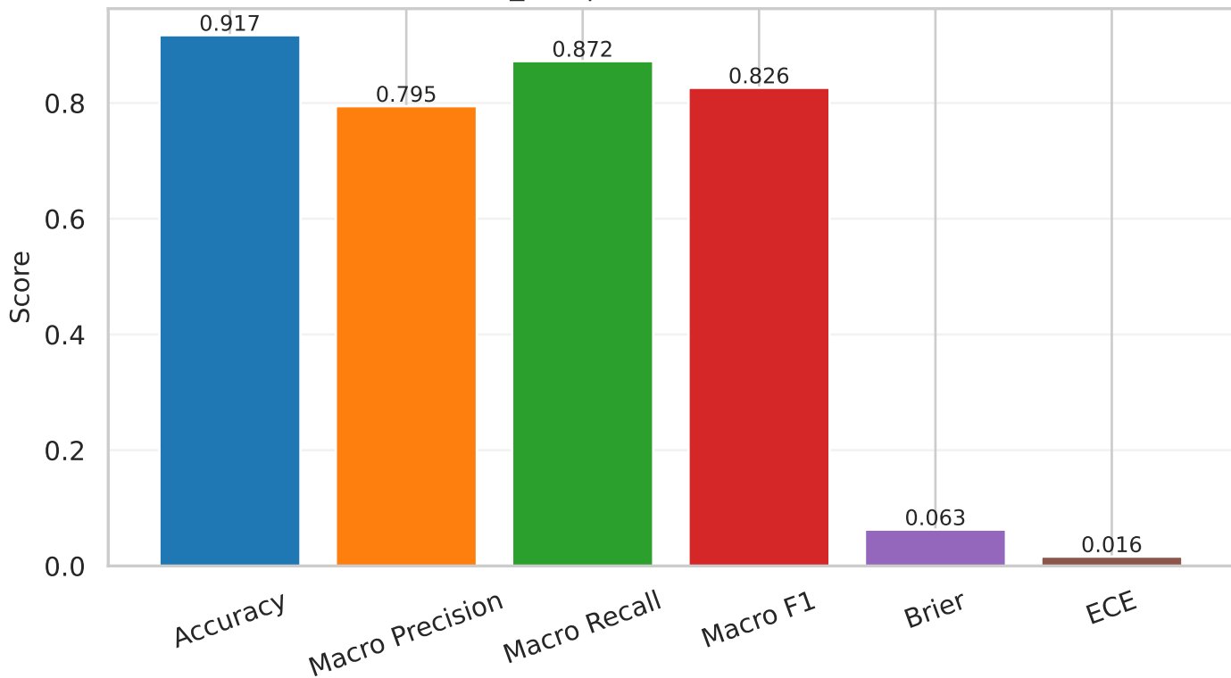
custom_cnn | val (calibrated) metrics
