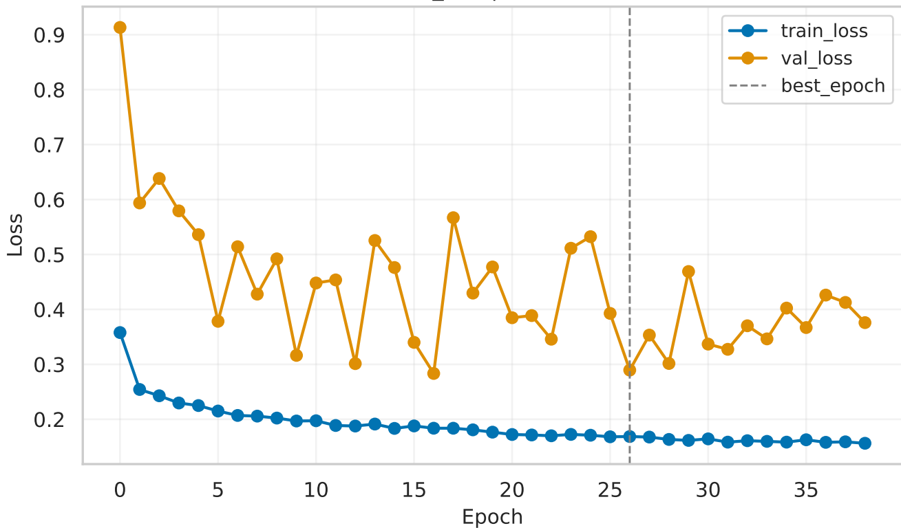
custom_cnn | Loss curves
