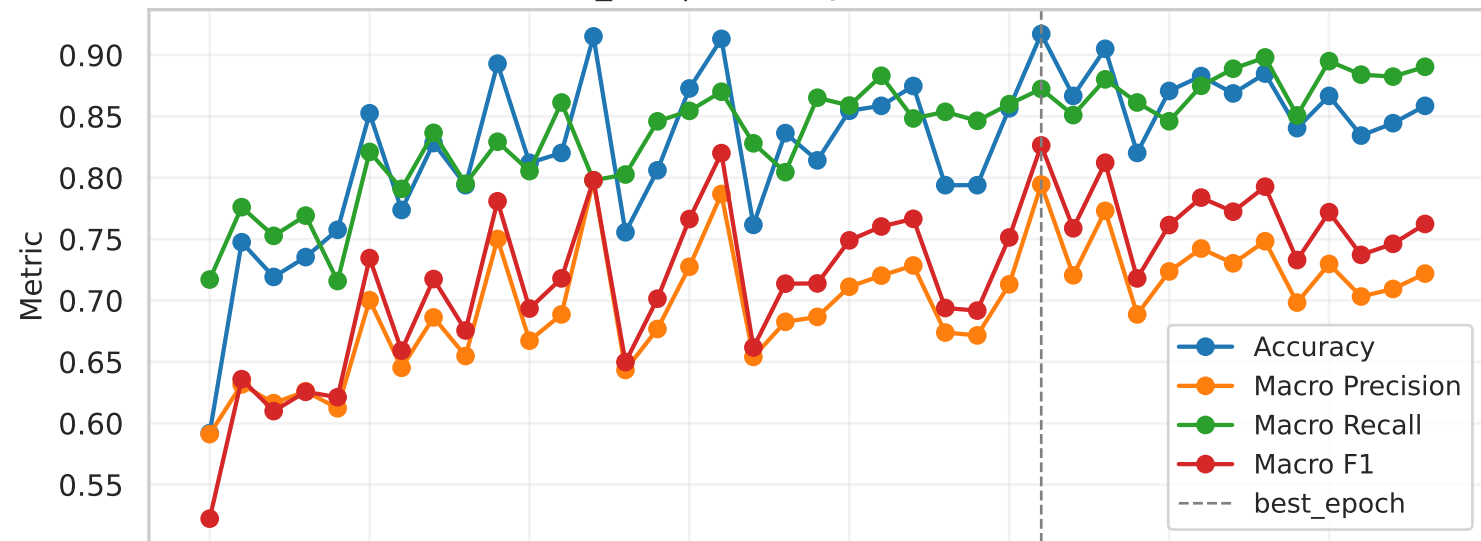
custom_cnn | Accuracy/Precision/Recall/F1
