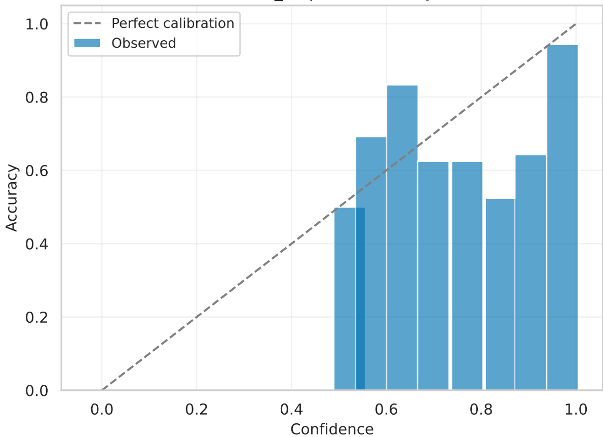
efficientnet_b1 | test Reliability (raw)
