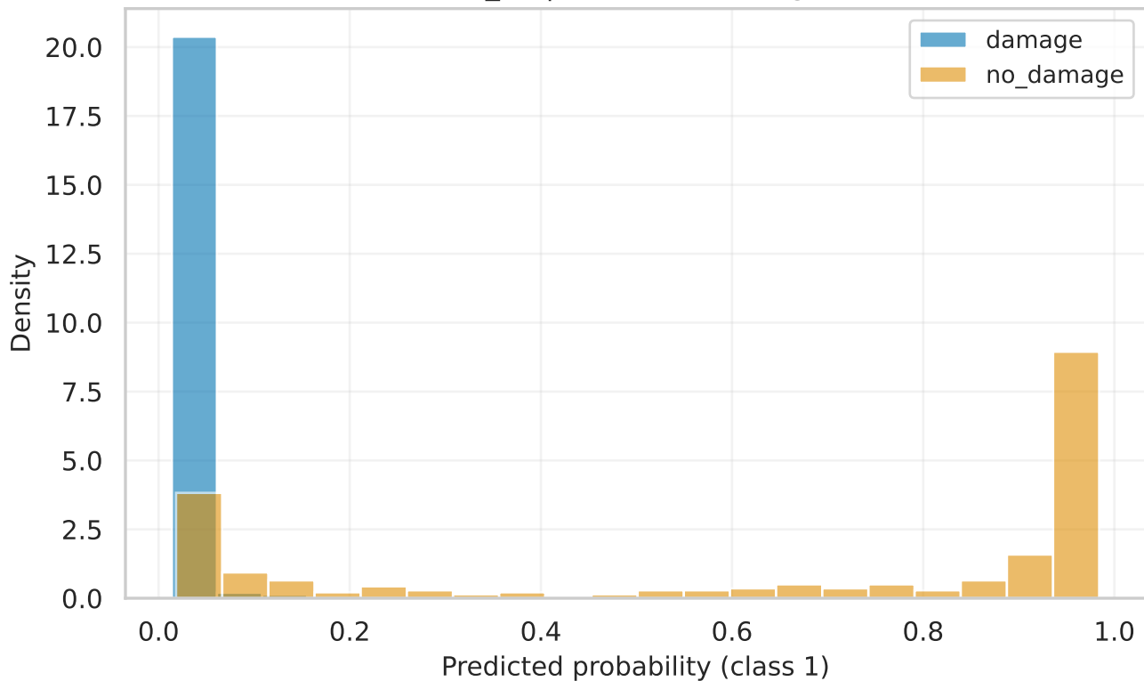
efficientnet_b1 | test Score Histogram (raw)
