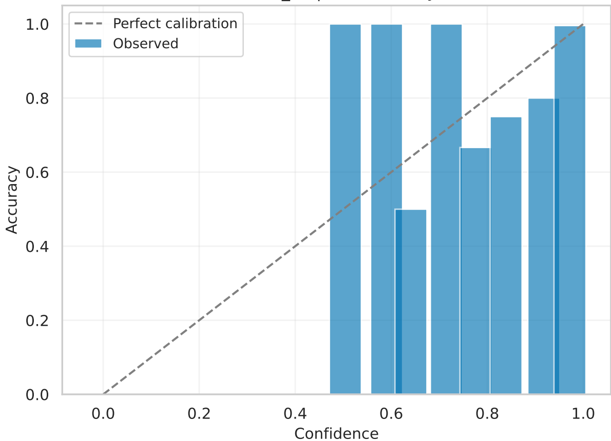
efficientnet_b1 | val Reliability (raw)
