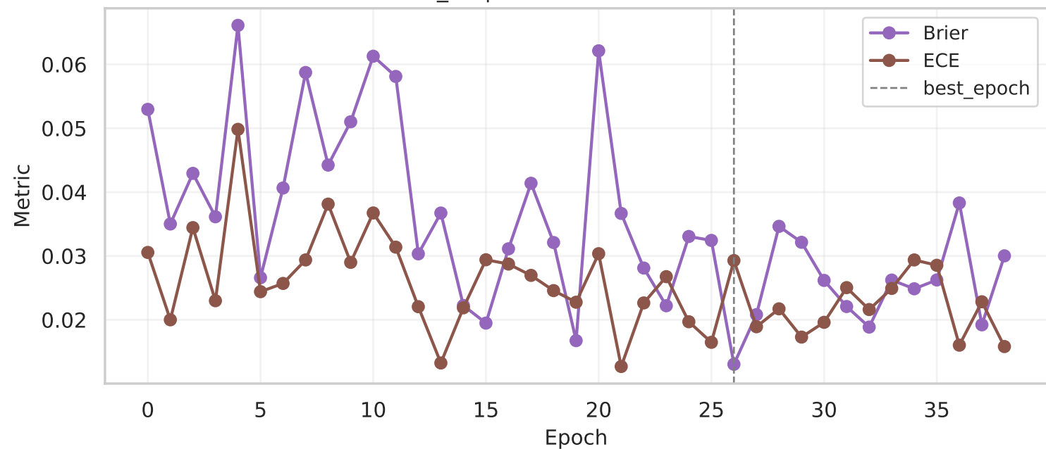
efficientnet_b1 | Calibration metrics (Brier/ECE)
