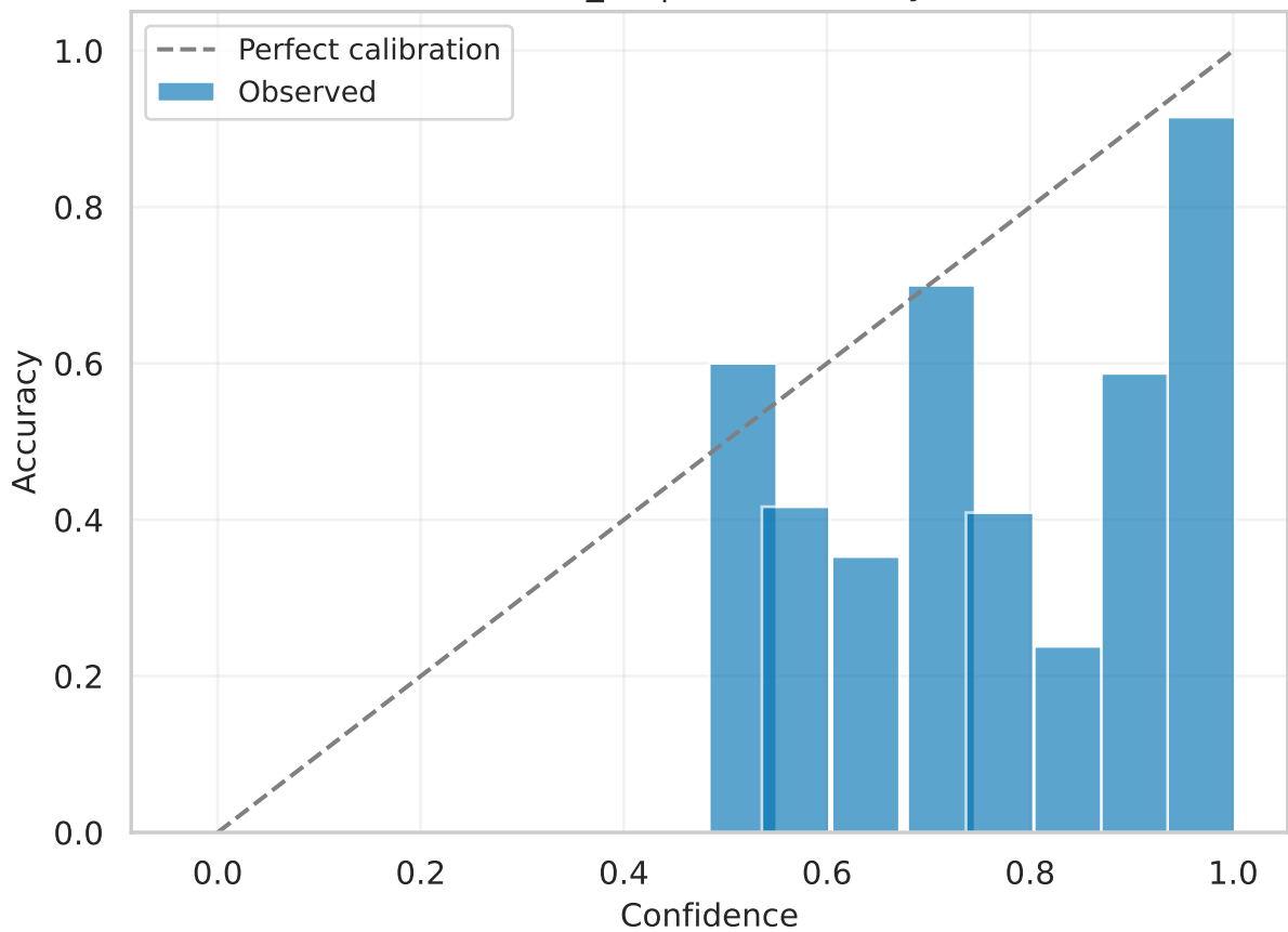
efficientnet_b2 | test Reliability (raw)
