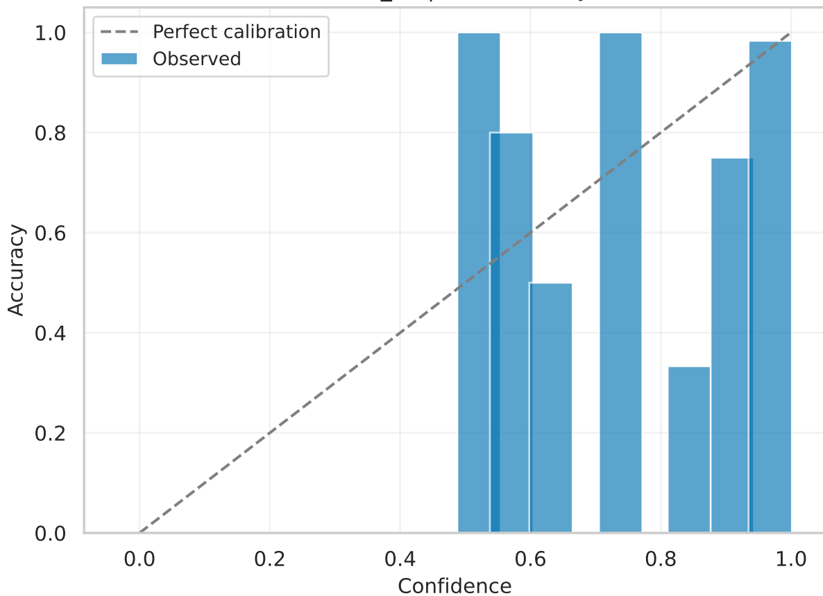
efficientnet_b2 | val Reliability (raw)
