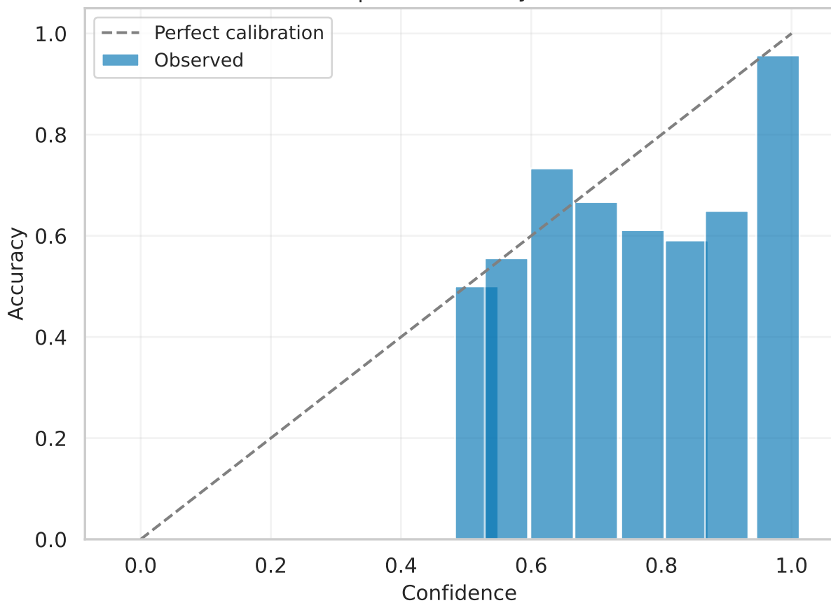
resnet18 | test Reliability (calibrated)
