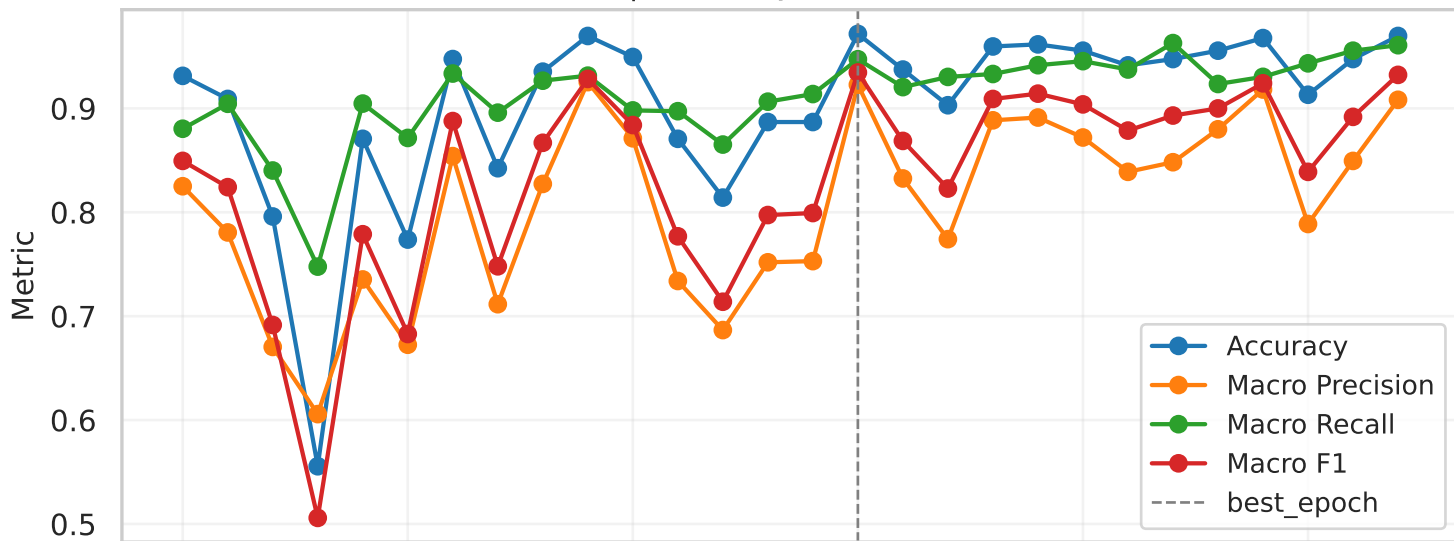
resnet18 | Accuracy/Precision/Recall/F1
