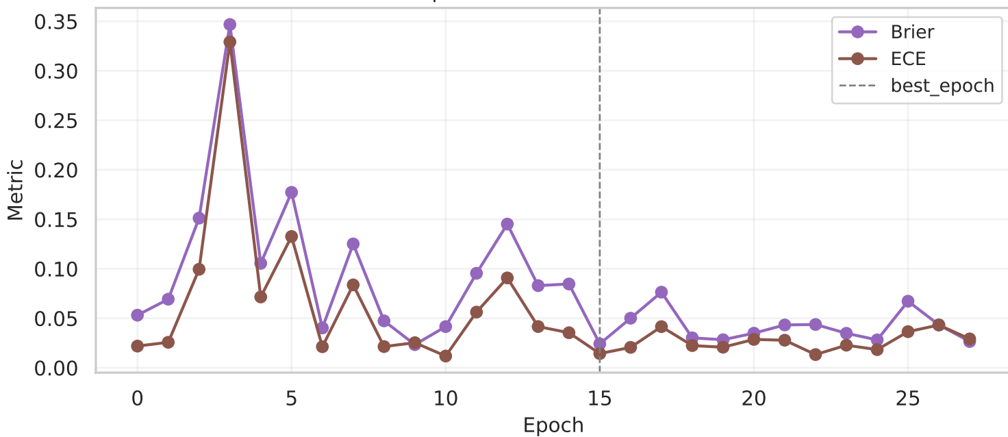
resnet18 | Calibration metrics (Brier/ECE)
