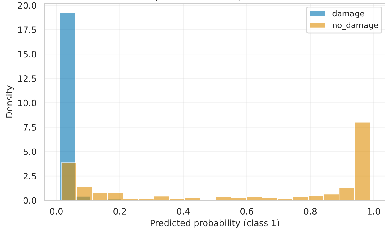
resnet34 | test Score Histogram (calibrated)
