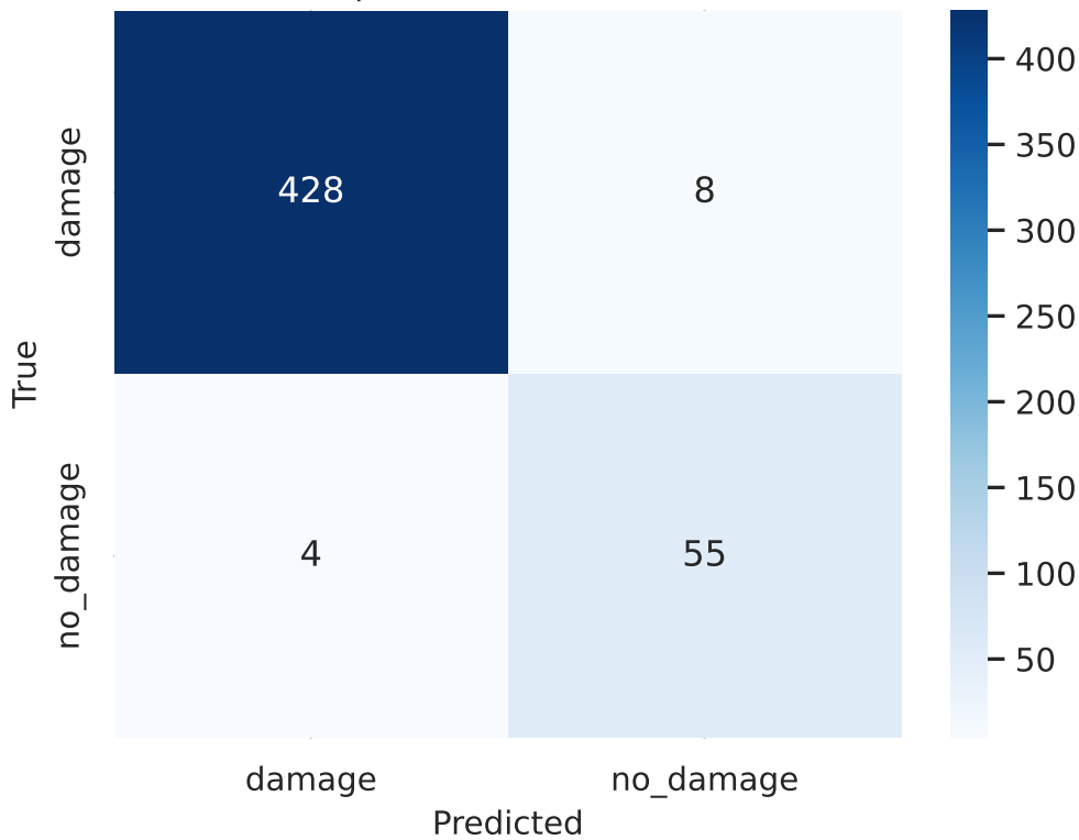
resnet50 | val Confusion (calibrated)
