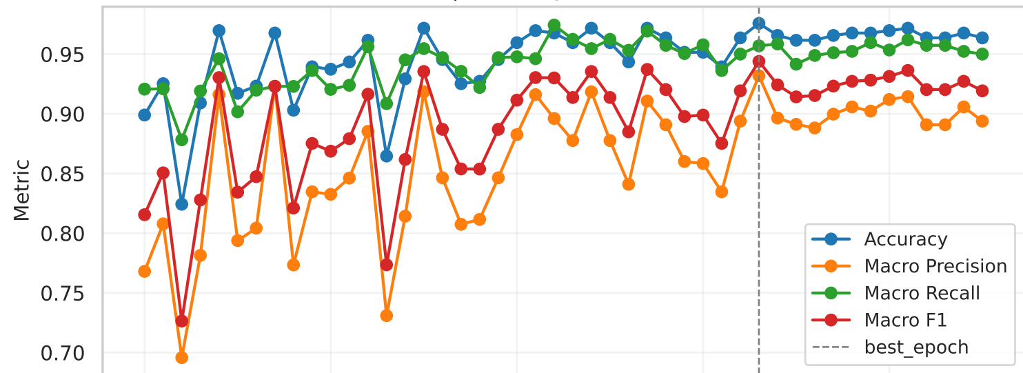
resnet50 | Accuracy/Precision/Recall/F1
