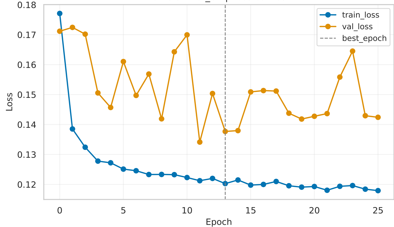
efficientnet_b2 | Loss curves
