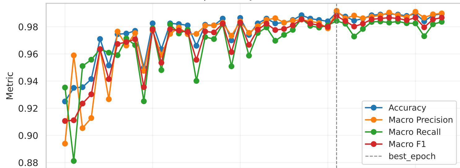
resnet18 | Accuracy/Precision/Recall/F1
