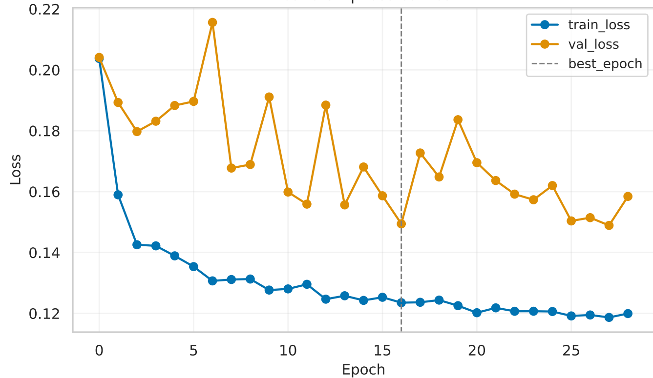
resnet34 | Loss curves
