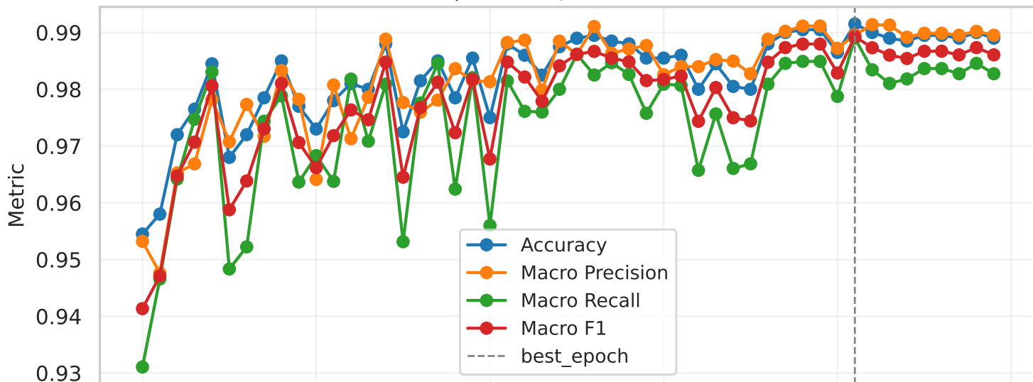
resnet50 | Accuracy/Precision/Recall/F1
