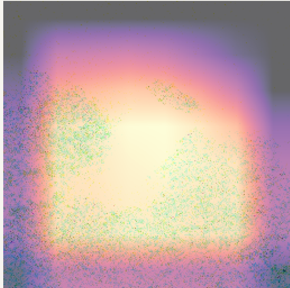
ResNet50 (Trained on Resampled Data) Resampled set Truth: Damage Damage confidence: 0.90
