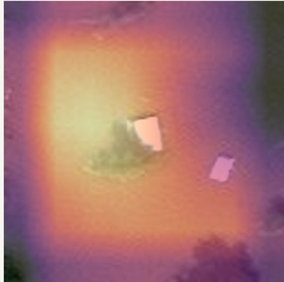
ResNet50 (Trained on Resampled Data) Resampled set Truth: Damage Damage confidence: 0.97
