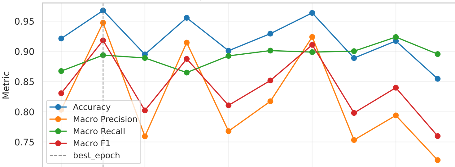
resnet34 | Accuracy/Precision/Recall/F1
